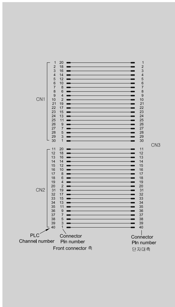
DHH40-□K25L
